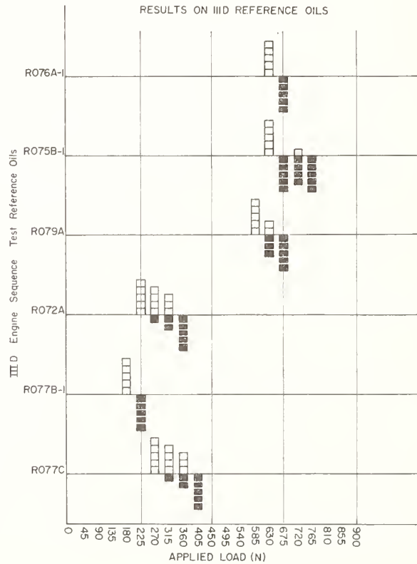
Figure 5. Modified Timken test results on six IIID engine sequence test oils. \square indicates pass test and \blacksquare denotes a failure. For each oil, five consecutive passes determines the maximum pass load and five consecutive failures indicates the minimum failure load.
